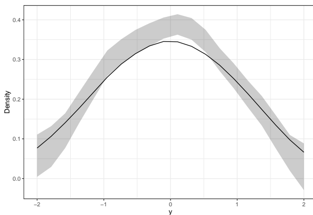
Figure 2: A simple density plot with robust 95% confidence bands.
